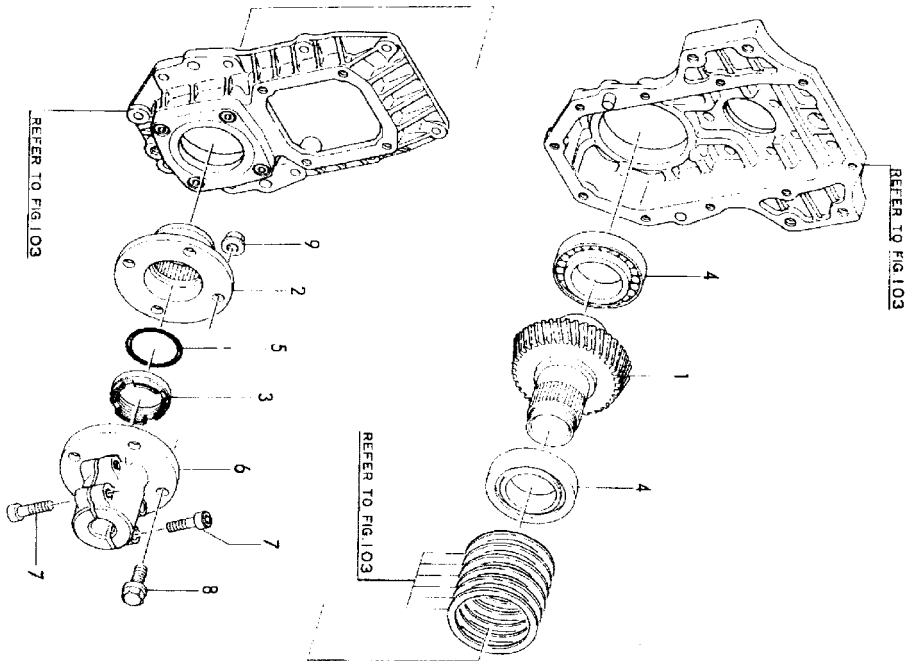
Fig. 107 V-DRIVE SHAFT
