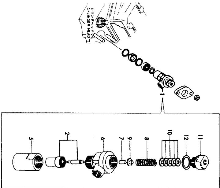
Fig. 45 燃料噴射弁 FUEL INJECTION VALVE
