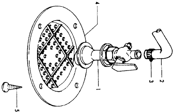
Kingston Cock (オプション) KINGSTON COCK (OPTIONAL)
