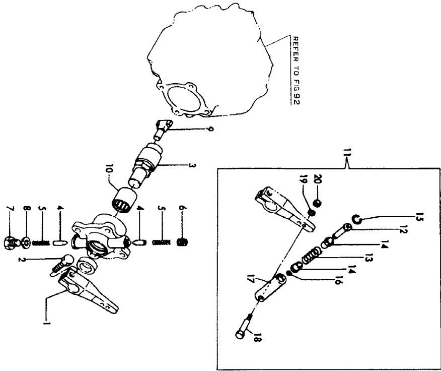
Fig. 95 操縦装置 REMOTE CONTROL DEVICE
